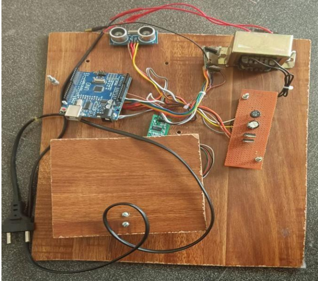
Figure 4: Prototype for Dustbin robot
