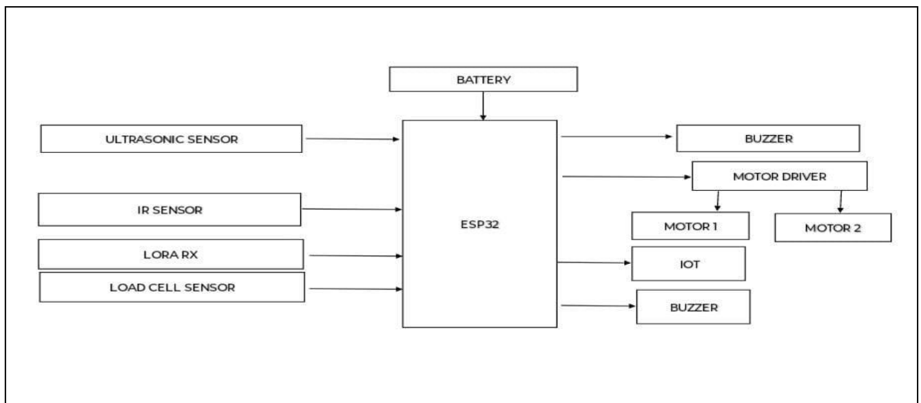
Figure 2: Transmitter Block diagram
